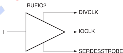
Figure 1-31: BUFIO2 Primitive
