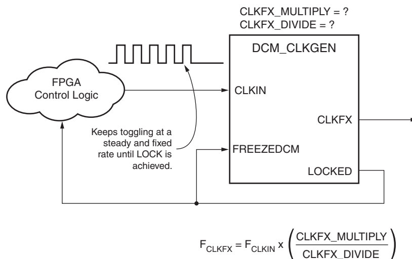
Figure 2-20: Setup of a Free-Running Oscillator
