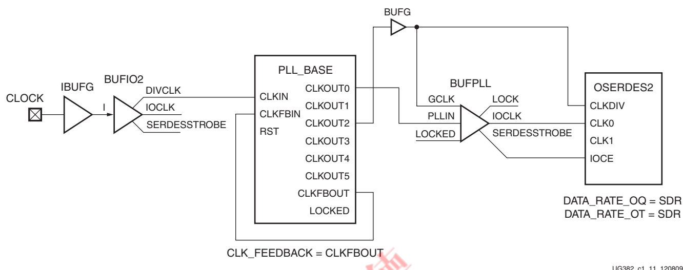
Figure 1-17: Example 4: Basic PLL OSERDES2 (SDR)
