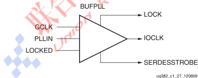
Figure 1-37: BUFPLL Primitive
