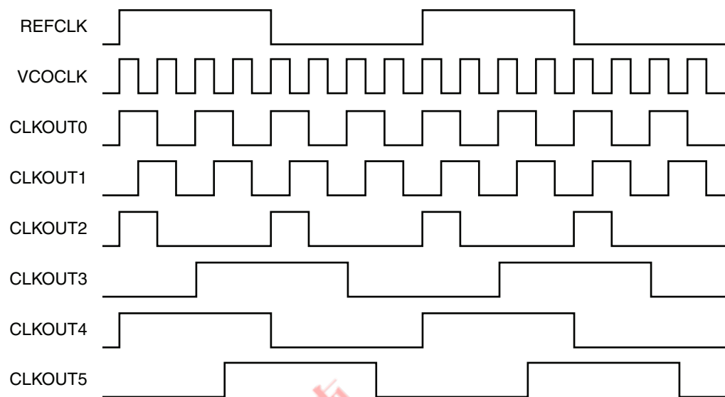
Figure 3-18: Example Waveform
