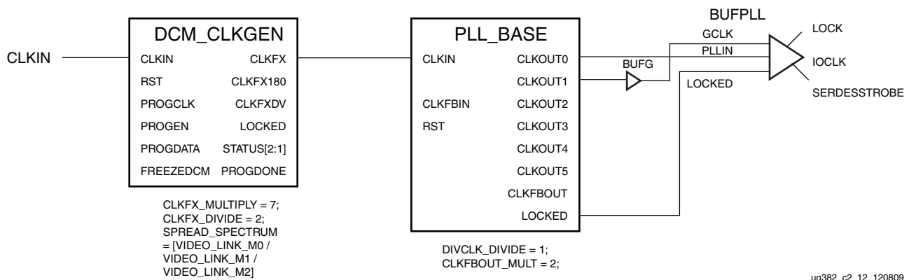
Figure 2-18: VIDEO_LINK Setup for Downspread Spread Spectrum 20-107 MHz (when F_{IN} \times 3.5 < \text{CLKOUT\_FREQ\_FX} )
