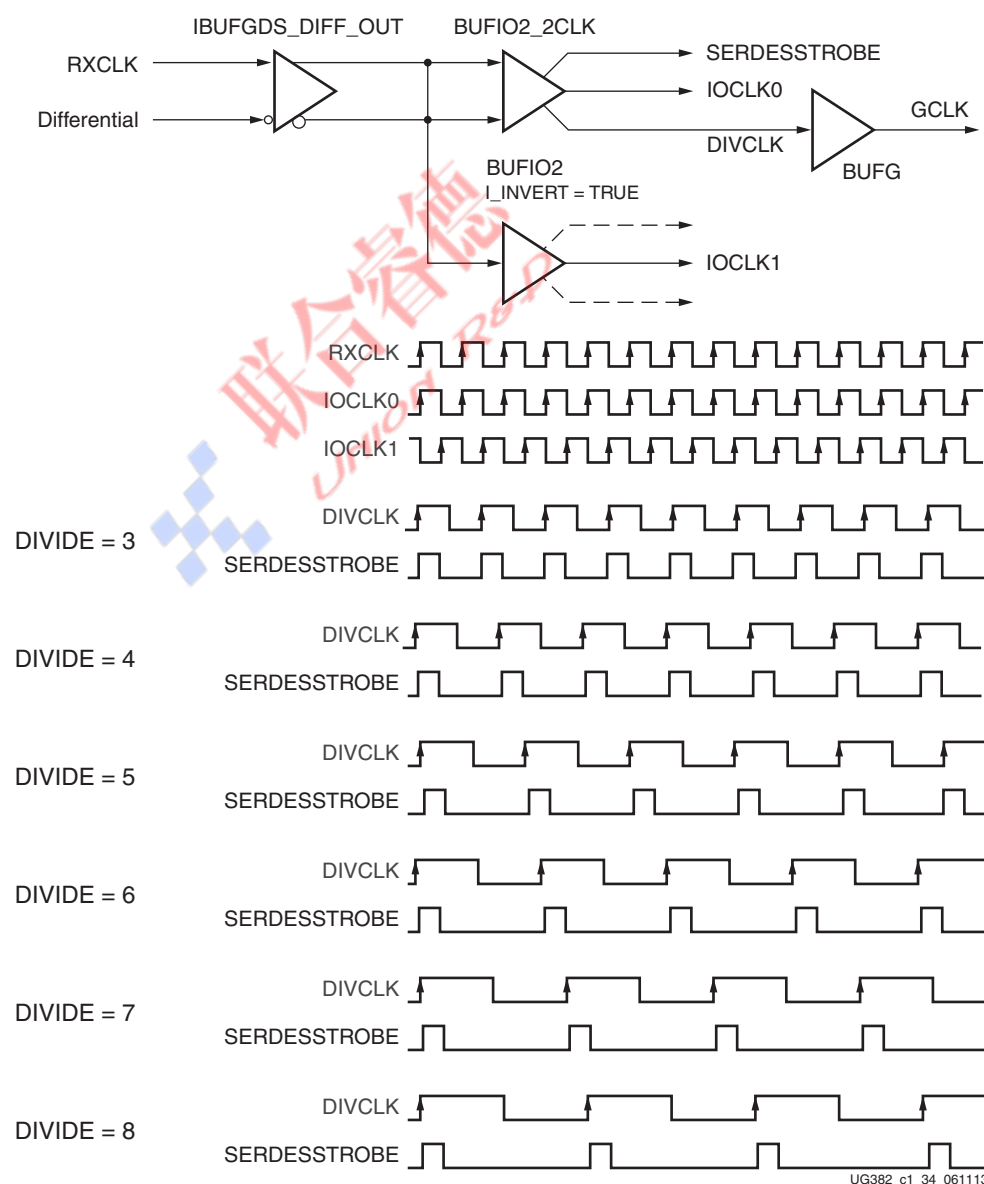
Figure 1-36: BUFIO2_2CLK Double Data Rate Clock
