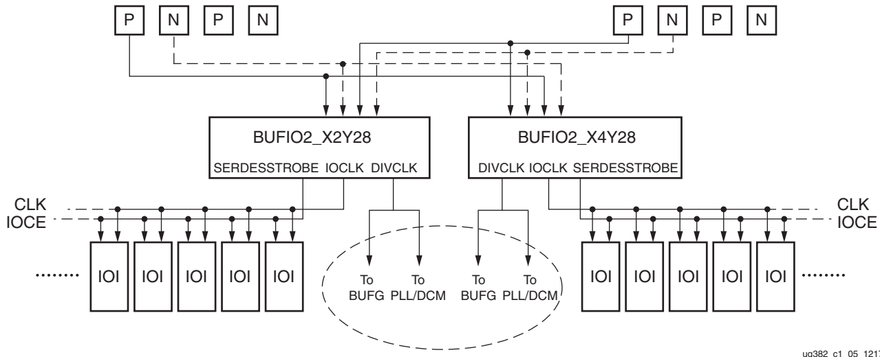
Figure 1-8: Dedicated Clock Inputs Routed by BUFIO2
