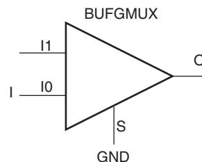
Figure 1-26: BUFG Built from a BUFGMUX
