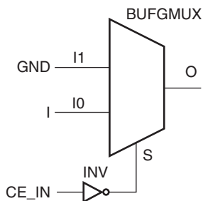
Figure 1-28: Equivalent Functionality of BUFCE
