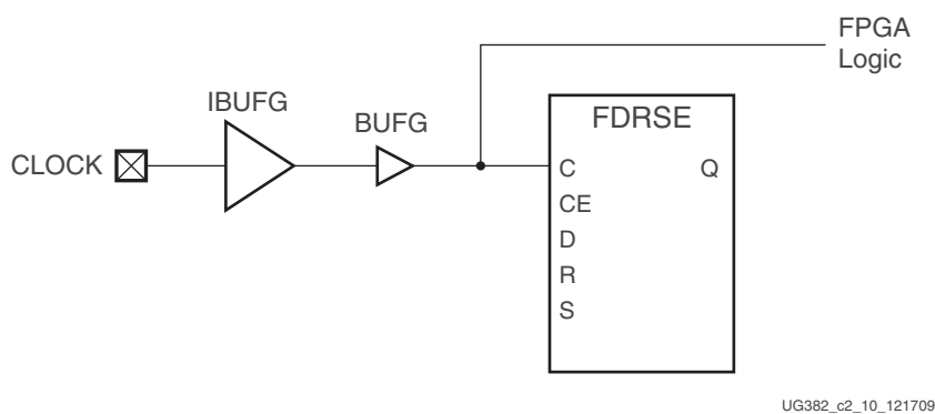
Figure 1-13: I/O Flip-Flop Clocking using BUFG
